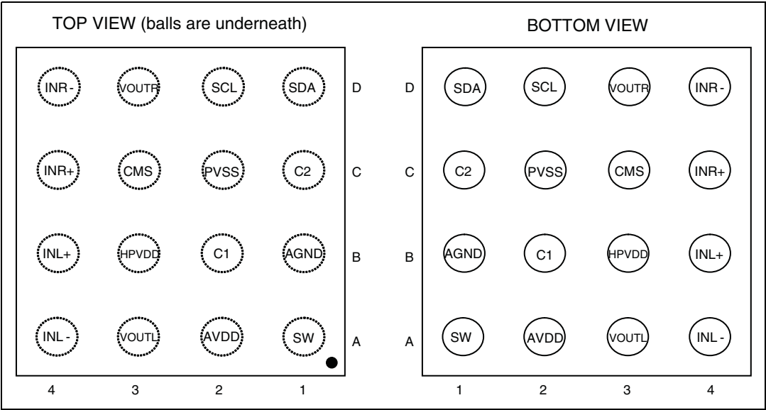
Figure 88. Pinout
